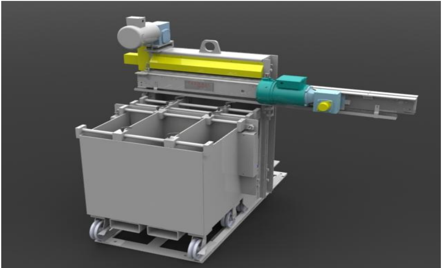
FEEDALL Model 3000 Hopper Feeder with Detachable Hopper for Centerless Grinding
